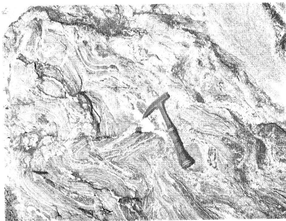
(a) and (b) Typical textures in hornblende migmatites, near Emurualigui
