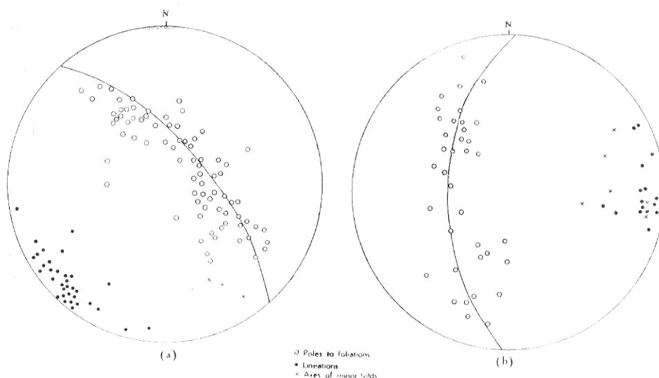
Fig. 4—(a) Structural data of the area south of Lodwar.
