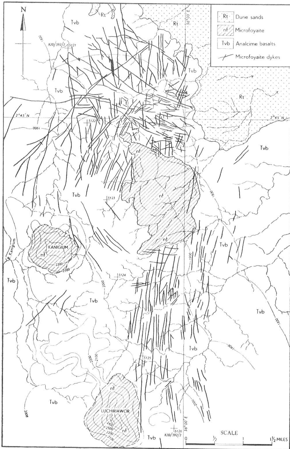
Fig. 2—Dyke swarm in the Kamutile Hills
