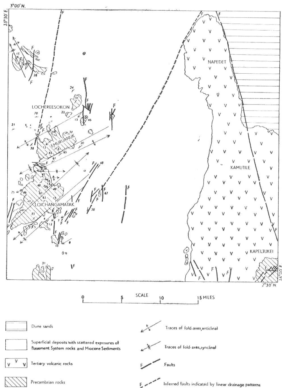
Fig. 3—Structural sketch-map of the area south of Lodwar.
