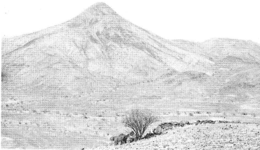
(b) Kamutile peak, a microfayaite plug
