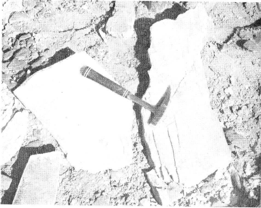
(a) Plates of gypsum (selenite) north of Lomenyangaparat gorge
