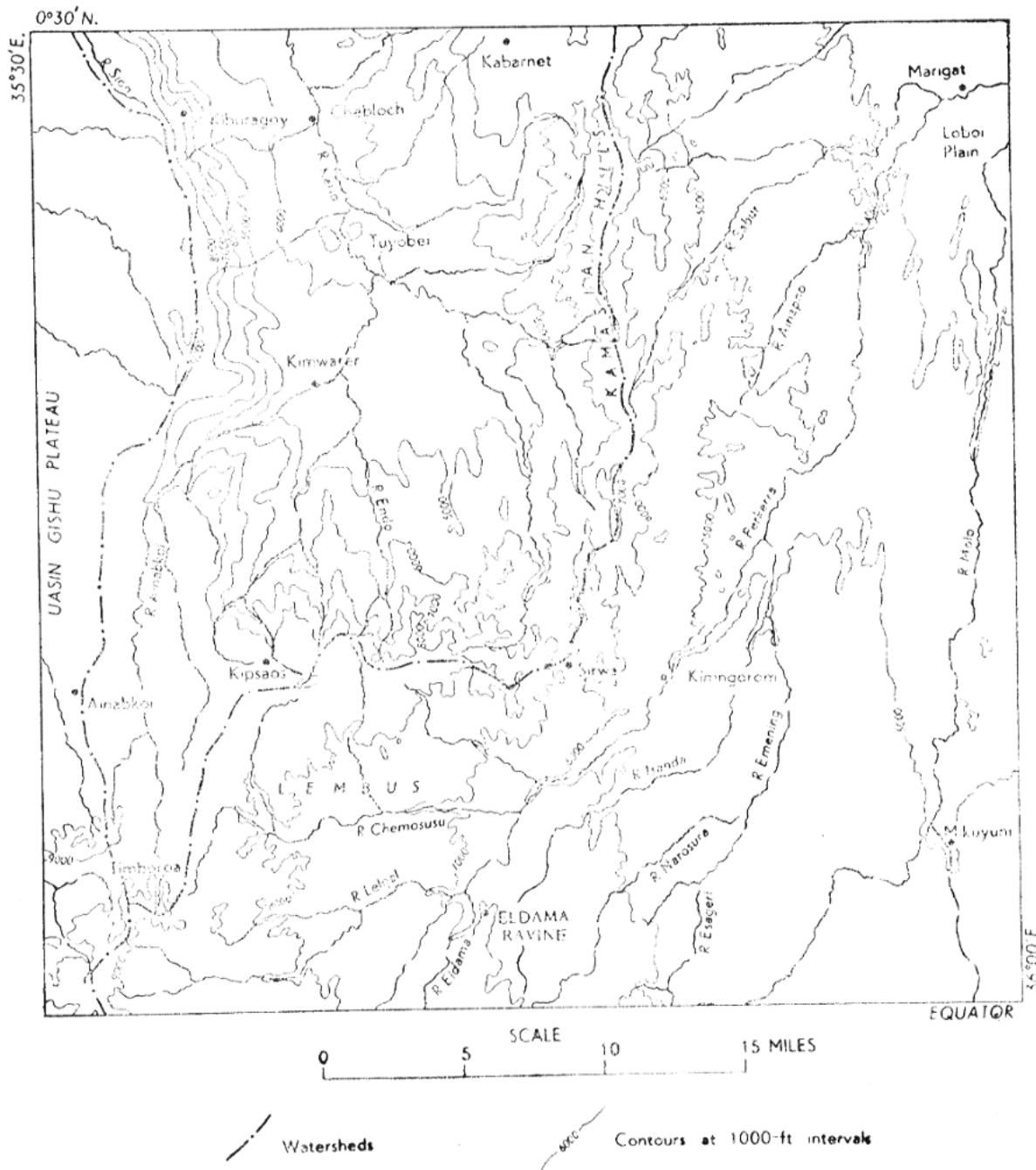
Fig. 2—Physiography of the Eldama Ravine-Kabarnet area
