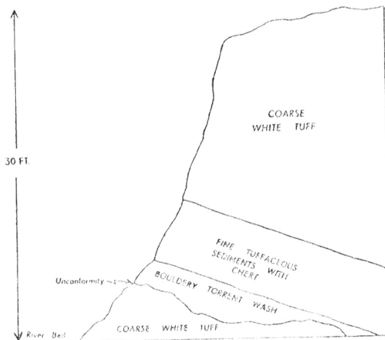
Fig. 4—Diagrammatic section of Eldama Ravine tuffs and sediments in the bank of the Perkerra River, north of Isanda
