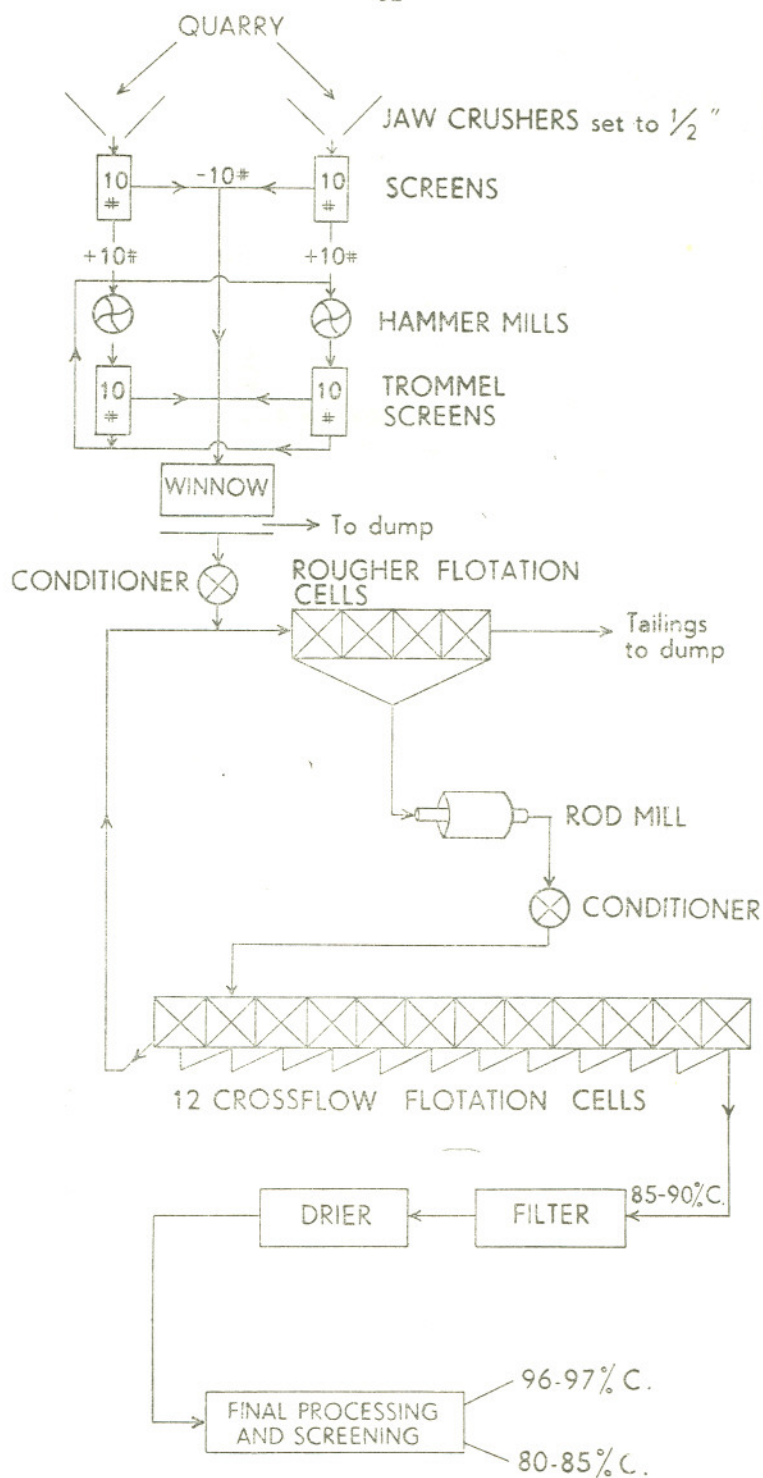
Fig. 6—Experimental graphite flow-sheet—Ganesh Claims, Kamstol
