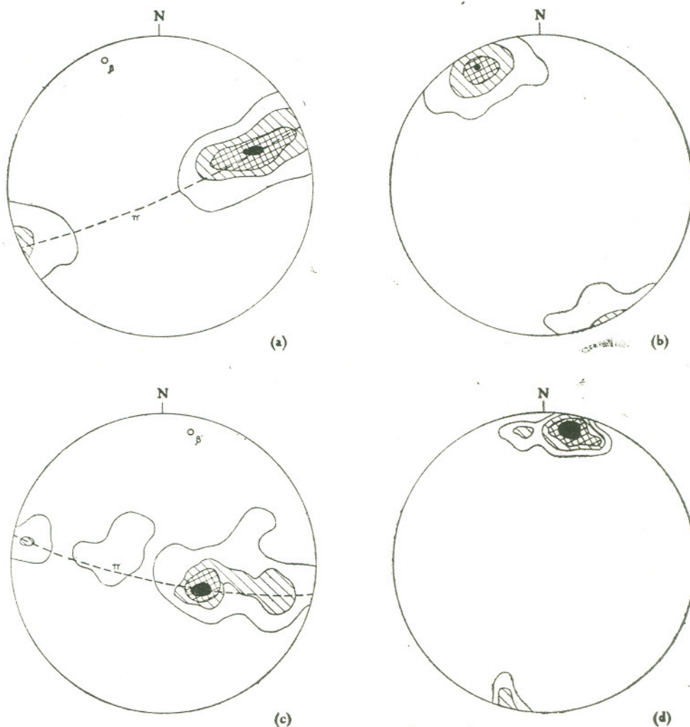
Fig. 3—Contoured stereographic diagrams of poles to foliation planes and of lineations in the Ikutha area:—
