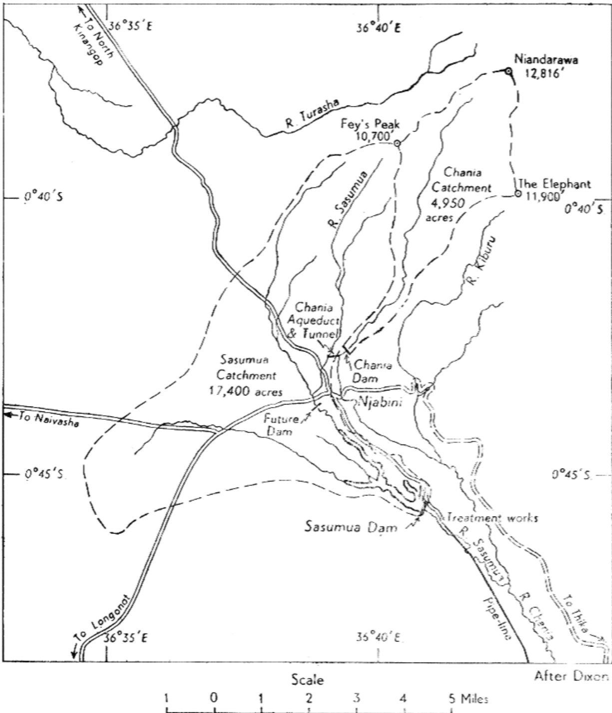
Fig. 6—The location of the Sasumua Dam
