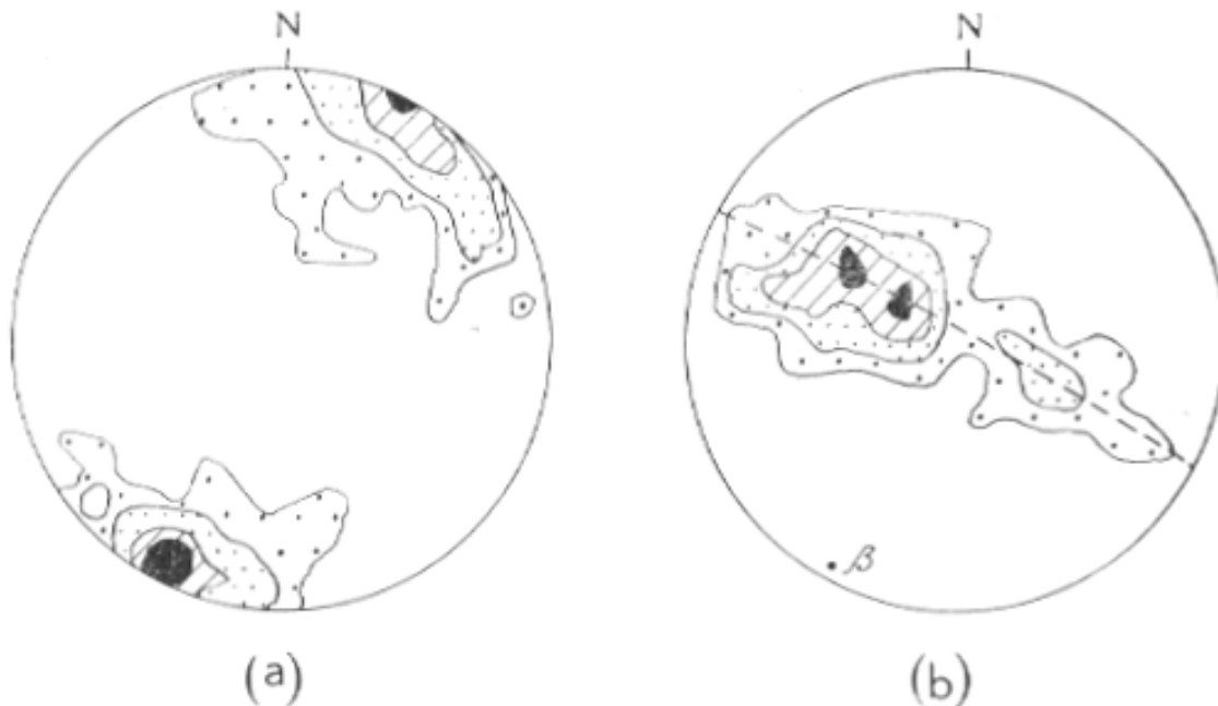
Fig. 4.—(a) Contoured diagram of stereographic projection of all b-lineations measured in the Loperot area.
