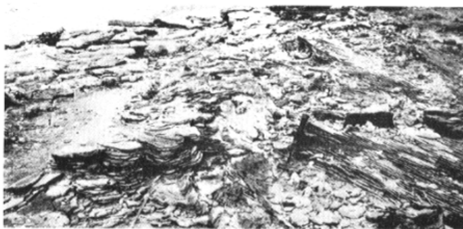
Plate III (c).—Folding and fracturing of incompetent laminated beds of the Turkana Grits in the Kalachir river channel.
