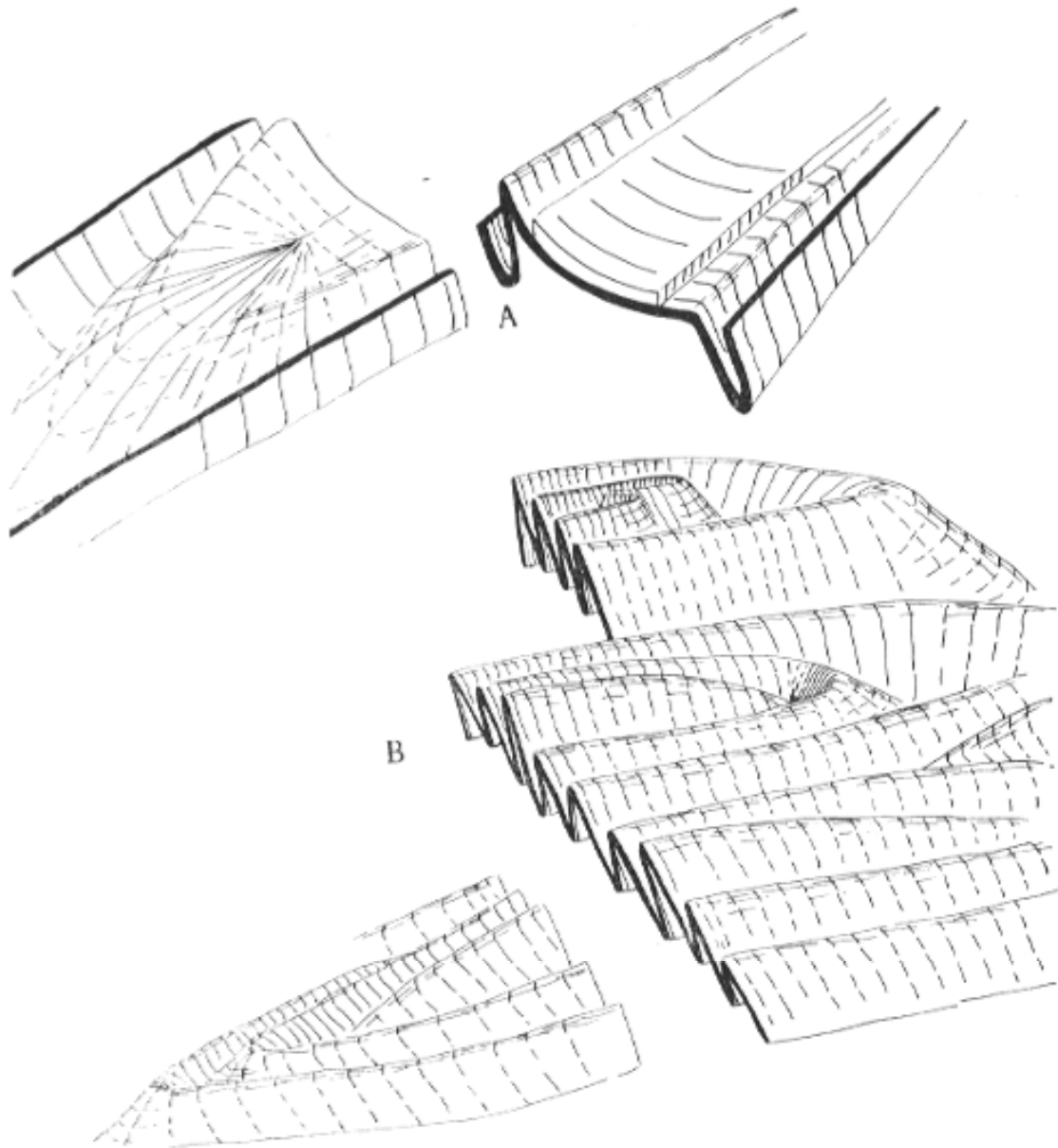
Fig. 5.—Idealized diagrams showing the nature of the folds:—
