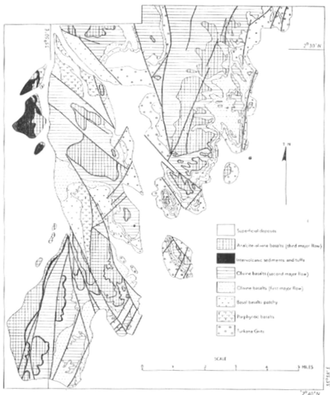
Fig. 2.—Map showing distribution of successive basaltic lava flows and intervolcanic sediments north of Loperot
