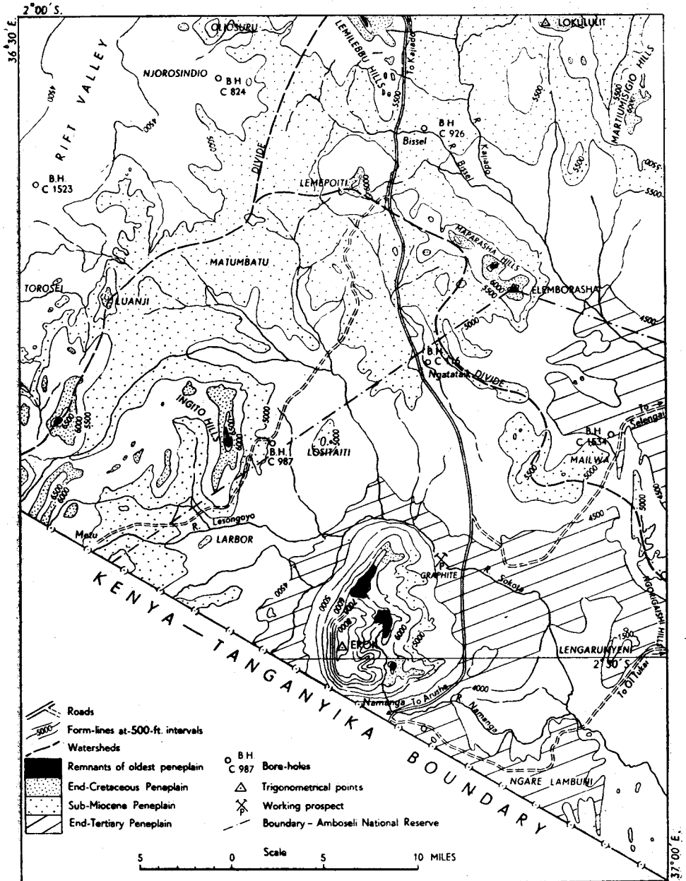
Fig. 1.—Physiographic sketch-map of the Namanga-Bissel area, showing also the location of water bore-holes and the situation of the graphite prospect in the Sokota valley.
