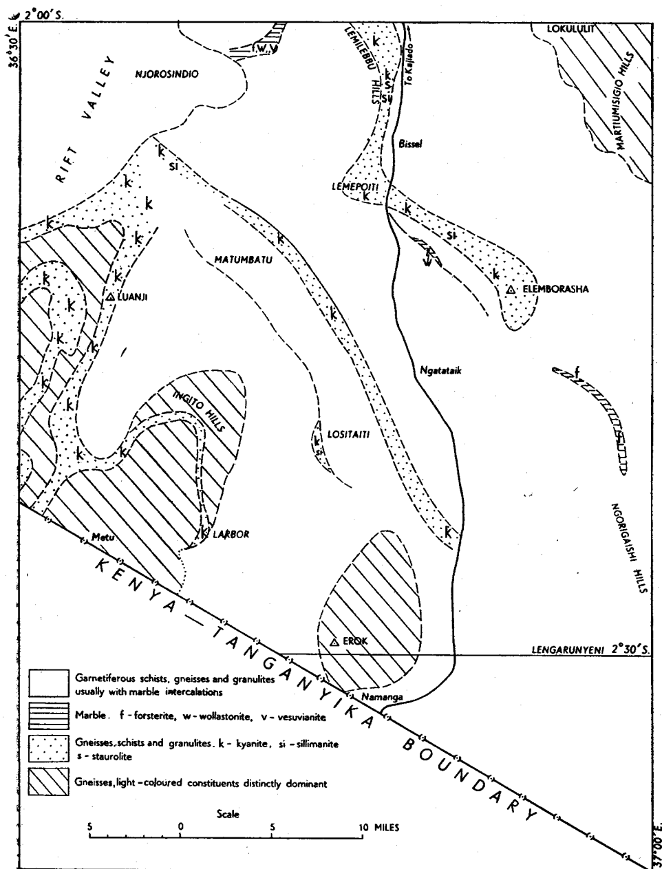
Fig. 2.—Metamorphic zones in the Basement System rocks of the Namanga-Bissel area.
