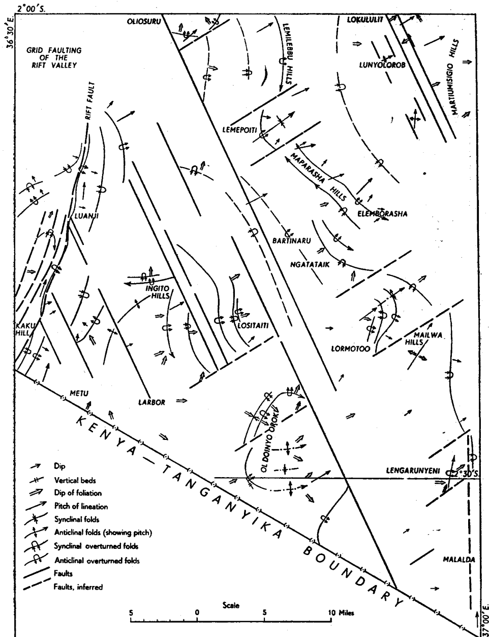
Fig. 3.—Structures in the Basement System in the Namanga-Bissel area. It should be noted that several inferred faults are shown that are not included on the geological map.
