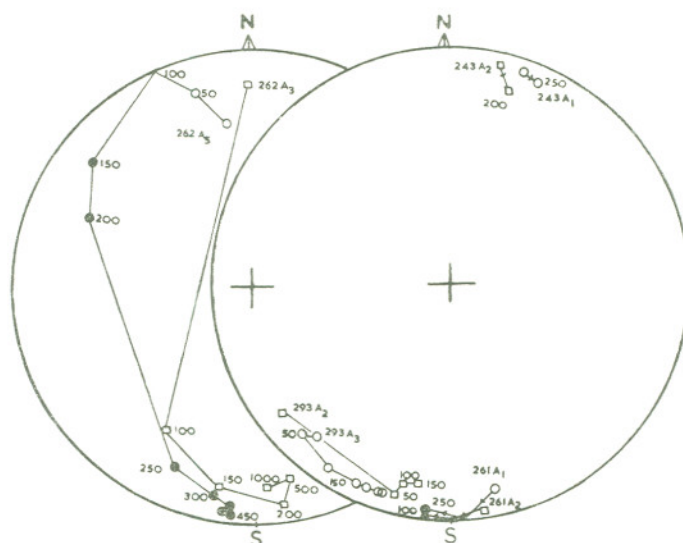
Fig. 1—Polar projection of typical changes of direction during demagnetization. ●, Dips down; ○, dips up: thermal demagnetization—numbers indicate temperatures in °C. ■, Dips down; □, dips up: alternating field demagnetization—numbers indicate peak field in oersteds
