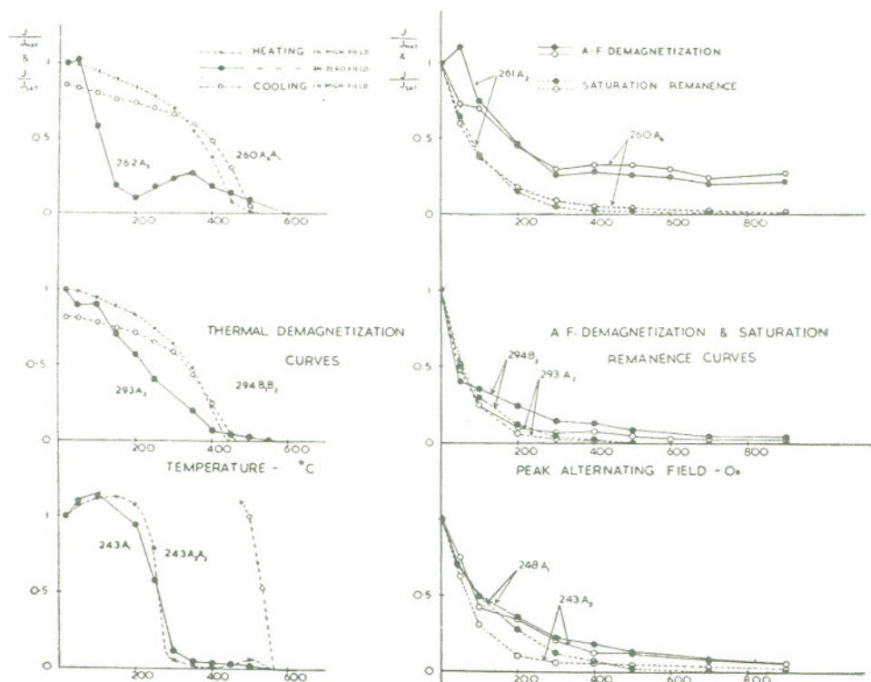
Fig. 2—Behaviour typical of dated sites during thermal and alternating-field demagnetization of natural remanent magnetism, alternating-field demagnetization of saturation remanence and high-field heating and cooling curves
