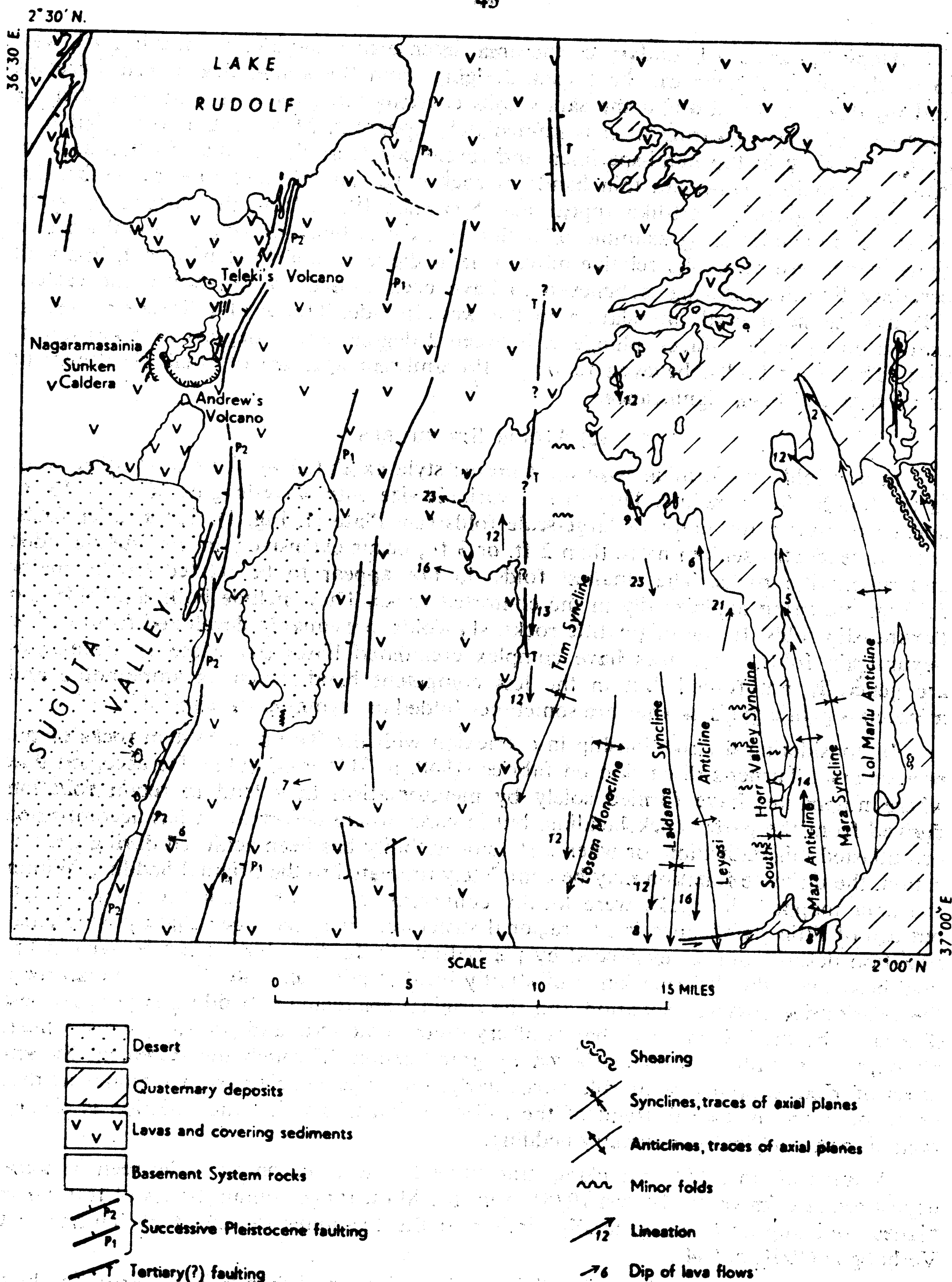
Fig. 3—Structural map of the South Horr area
