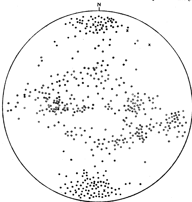
Fig. 4—Structural data from the Basement System rocks plotted on the lower hemisphere of a Schmidt equal area net
