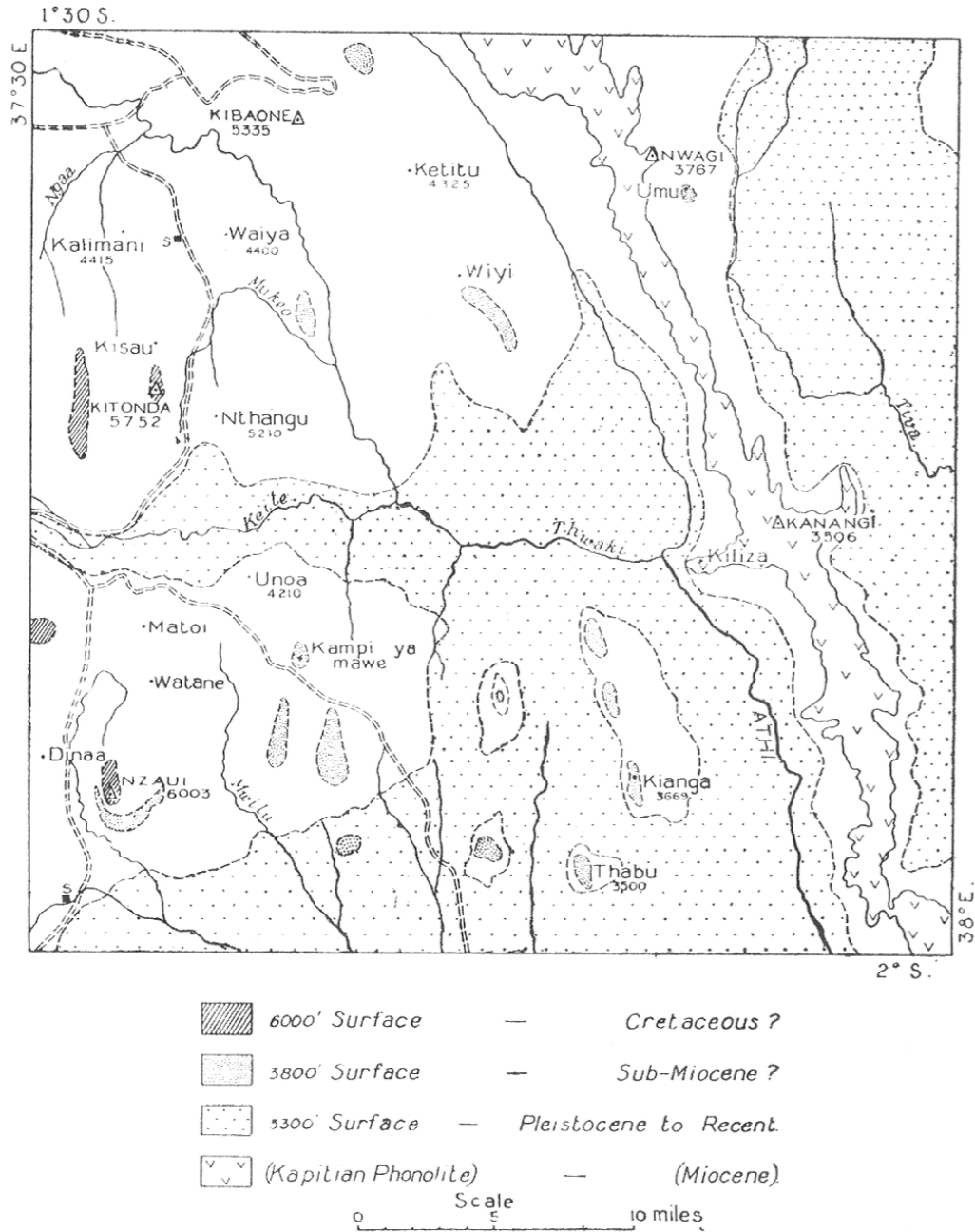
FIG. 1.—Erosion surfaces in the south-east Machakos area.
