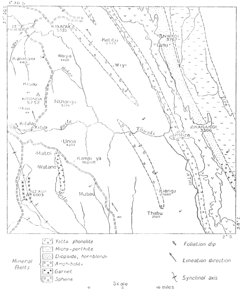
FIG. 2.—Structures and mineral belts in the area south-east of Machakos.
