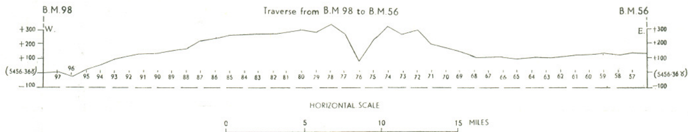
Fig. 3.—Graph showing profiles of the results of magnetometer traverses.
