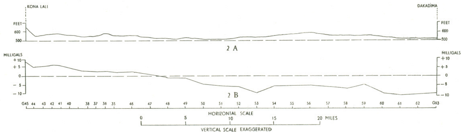
A=Elevation Profile B=Gravimetric absolute Bouguer Anomaly Profile Fig. 4.—Graph showing the gravimetric profiles of the traverse lines.
