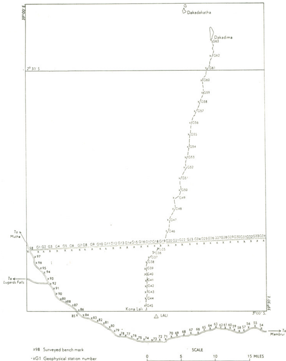
Fig. 2.—Map showing the geophysical traverses carried out in the Lali Hills-Dakadima area.
