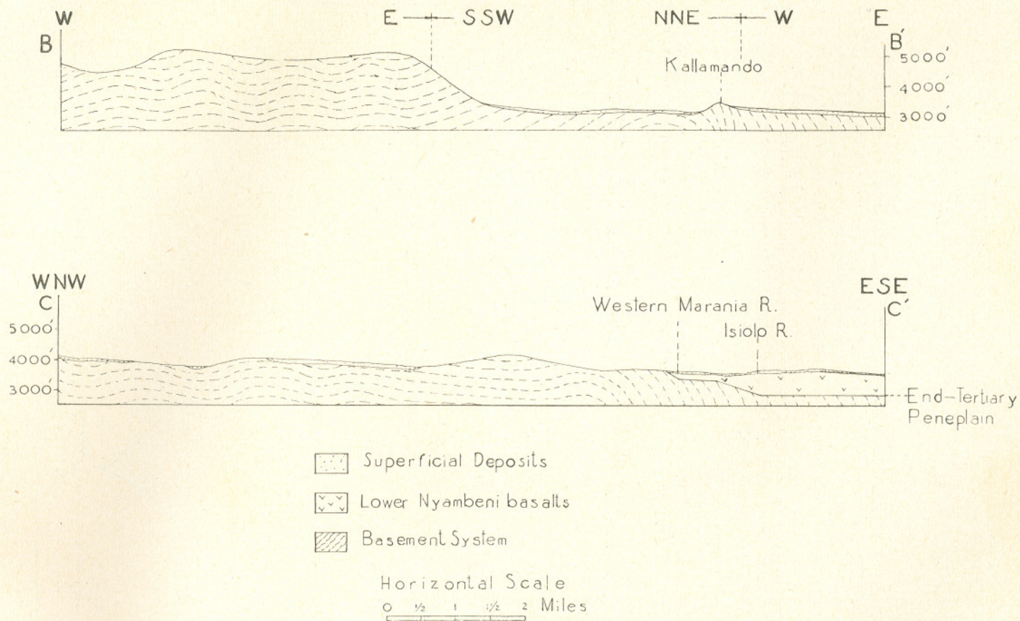
Fig. 4.—Geological cross-section to illustrate the structural axis in the Basement System rocks near Isiolo. The lines of section B-B' and C-C' are shown on the map.
